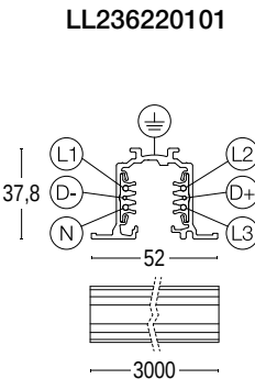
Binario tri-fase & Bus - Incassato Three-circuit tracks & Bus - Recessed
