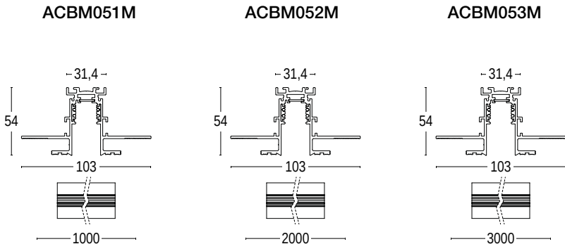
Binario BM05 R 48V Track BM05 R 48V
