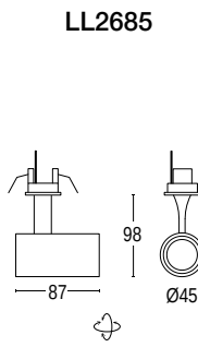
Point Evo 0R 45
