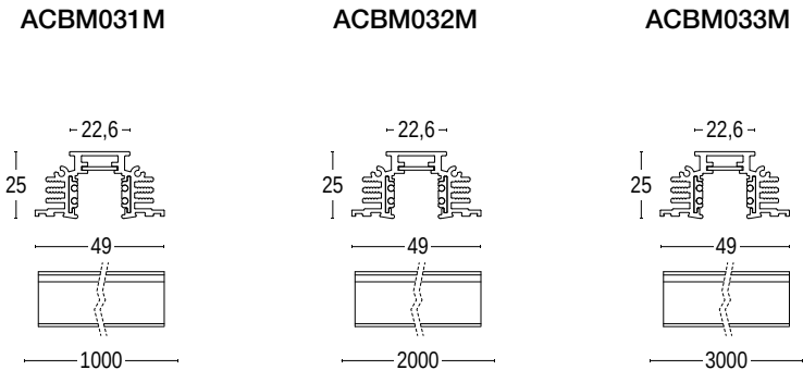
Binario BM03 R 48V Track BM03 R 48V
